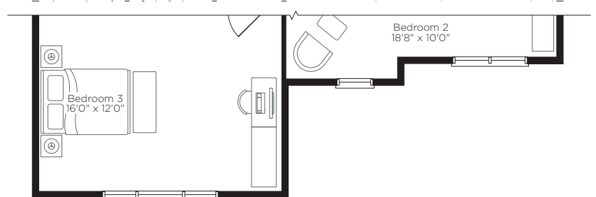
Partial Second Floor Elev. B
