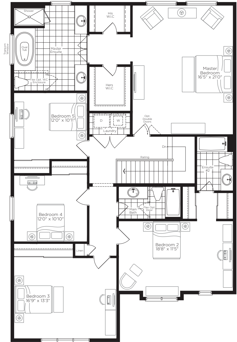
Second Floor w/5 Bedroom Option Elev. A & D
