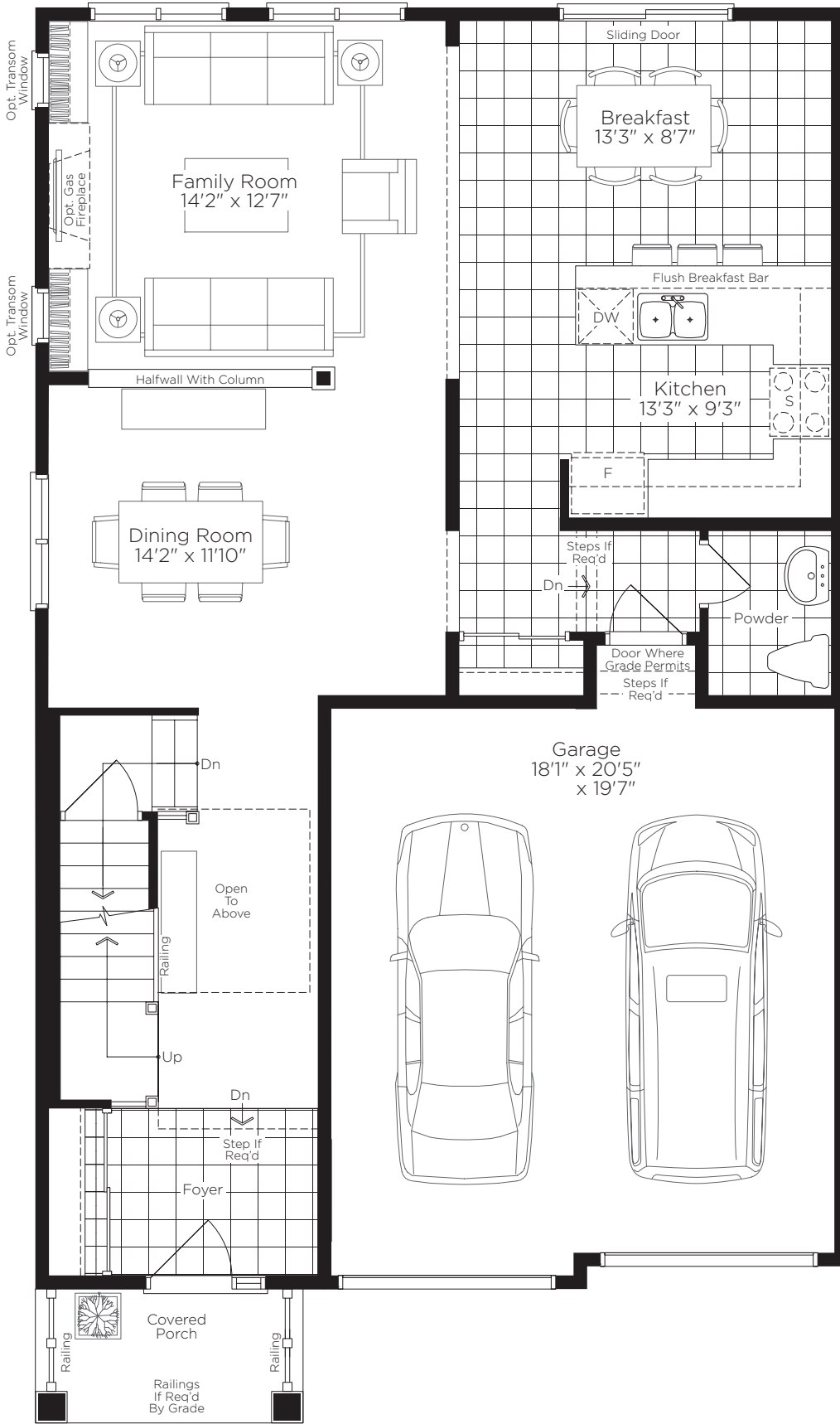
Ground Floor Elev. A, B & D
