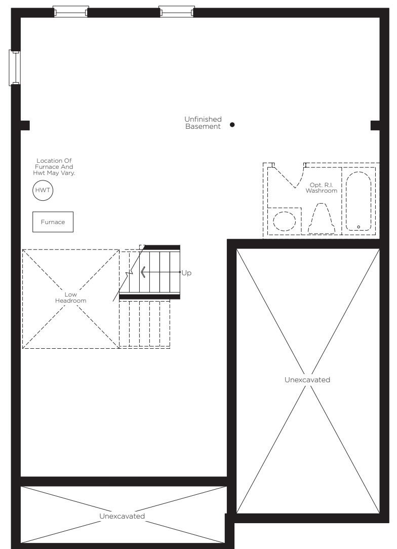
Basement Floor Elev. A & B
