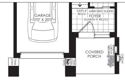
PARTIAL GROUND FLOOR PLAN ELEV. 'G'
