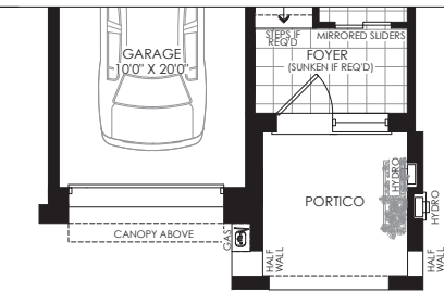
PARTIAL GROUND FLOOR PLAN ELEV. 'C'
