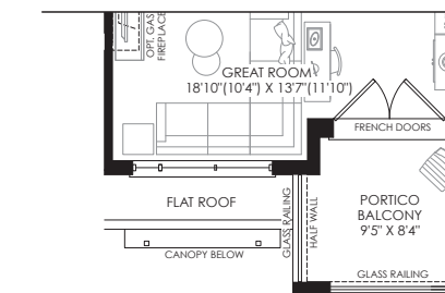
PARTIAL SECOND FLOOR PLAN ELEV. 'C'
