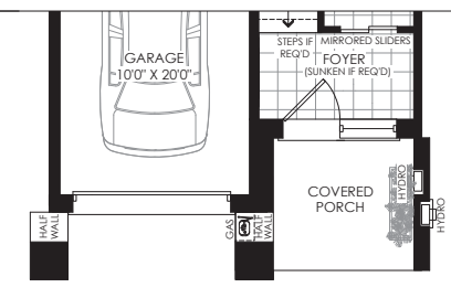
PARTIAL GROUND FLOOR PLAN ELEV. 'F'
