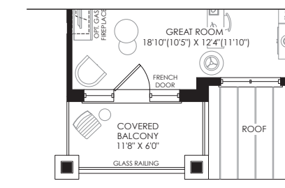
PARTIAL SECOND FLOOR PLAN ELEV. 'G'
