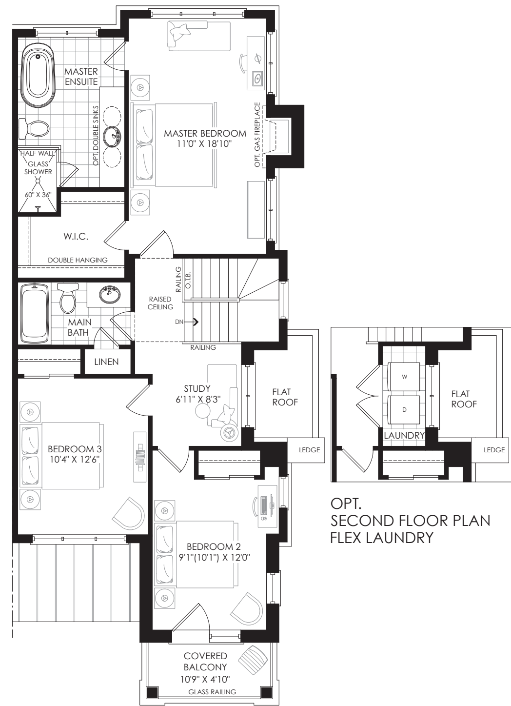
SECOND FLOOR PLAN ELEV. 'H'
