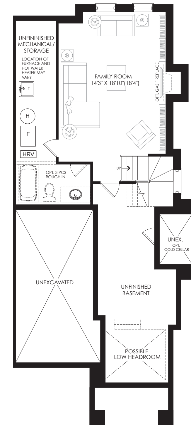
BASEMENT PLAN ELEV. 'H'
