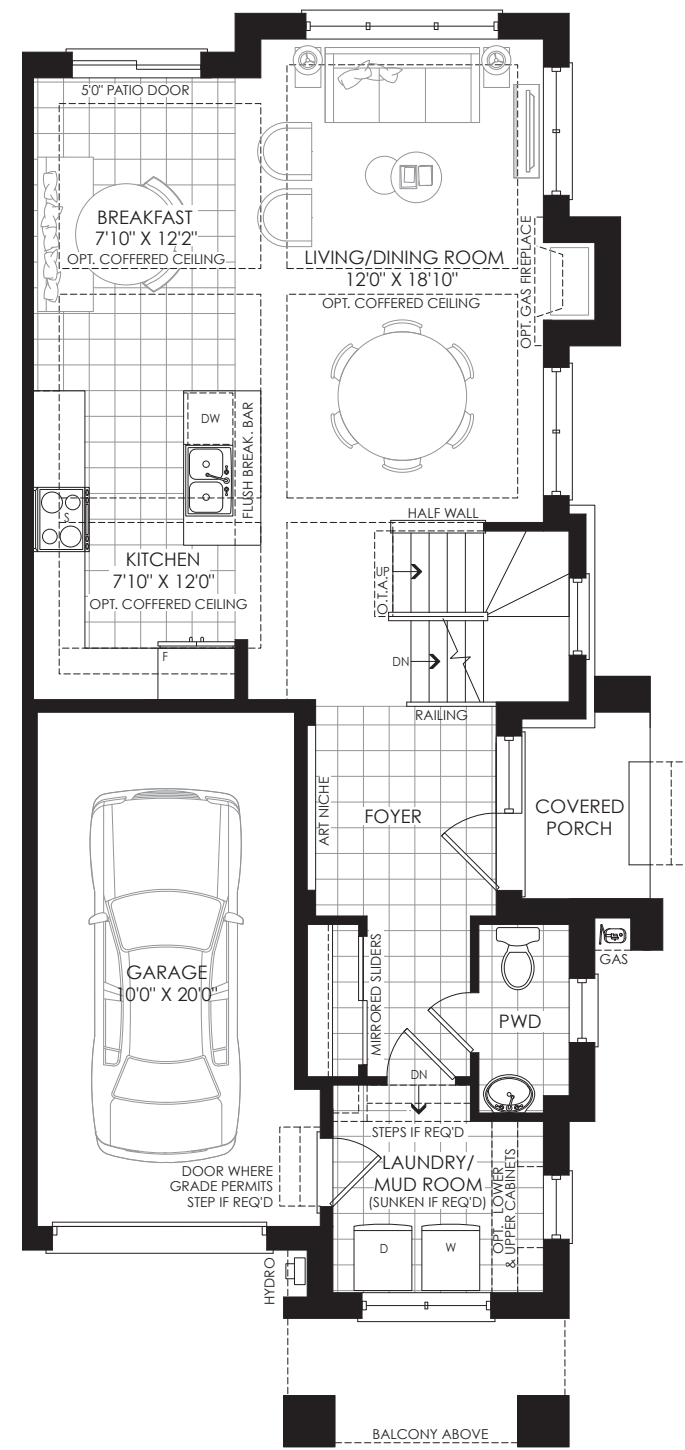
GROUND FLOOR PLAN ELEV. 'H'
