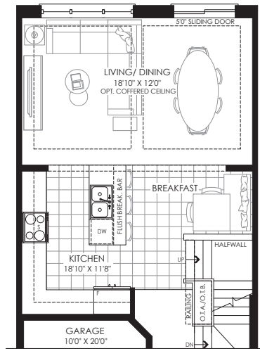
PARTIAL GROUND FLOOR FLEX PLAN
