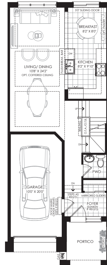
GROUND FLOOR PLAN ELEV. 'A'
