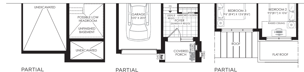
PARTIAL BASEMENT PLAN ELEV. 'F' PARTIAL GROUND FLOOR PLAN ELEV. 'F' PARTIAL SECOND FLOOR PLAN ELEV. 'F'
