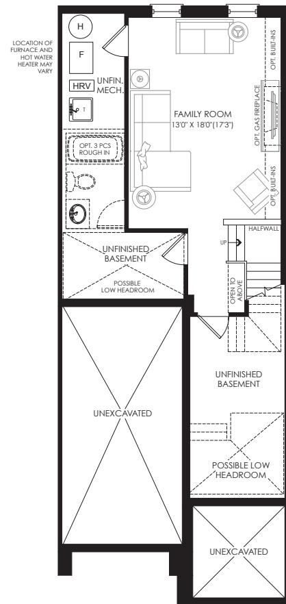
BASEMENT PLAN ELEV. 'A'
