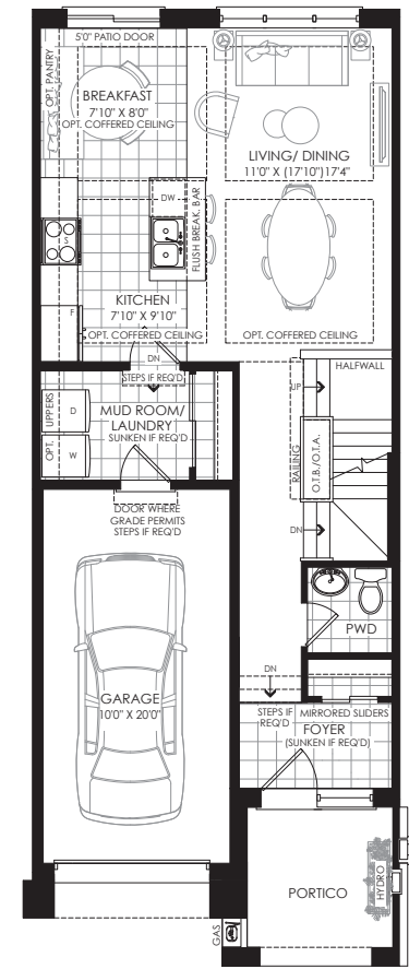
GROUND FLOOR PLAN ELEV. 'A'
