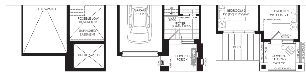
PARTIAL BASEMENT PLAN ELEV. 'G' PARTIAL GROUND FLOOR PLAN ELEV. 'G' PARTIAL SECOND FLOOR PLAN ELEV. 'G'
