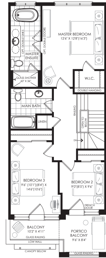
SECOND FLOOR PLAN ELEV. 'A'
