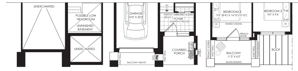
PARTIAL BASEMENT PLAN ELEV. 'E' PARTIAL GROUND FLOOR PLAN ELEV. 'E' PARTIAL SECOND FLOOR PLAN ELEV. 'E'
