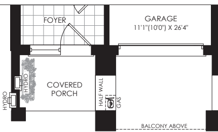
PARTIAL GROUND FLOOR PLAN ELEV. 'F'
