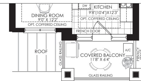
PARTIAL SECOND FLOOR PLAN ELEV. 'G'
