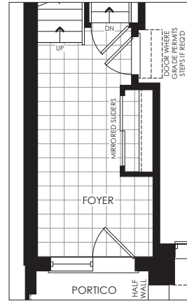
PARTIAL GROUND FLOOR PLAN FOR FLEX THIRD FLOOR WITH LAUNDRY
