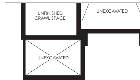
PARTIAL CRAWL SPACE PLAN ELEV. 'C'
