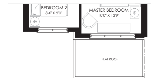
PARTIAL THIRD FLOOR PLAN / FLEX PLAN WITH LAUNDRY ELEV. 'G'
