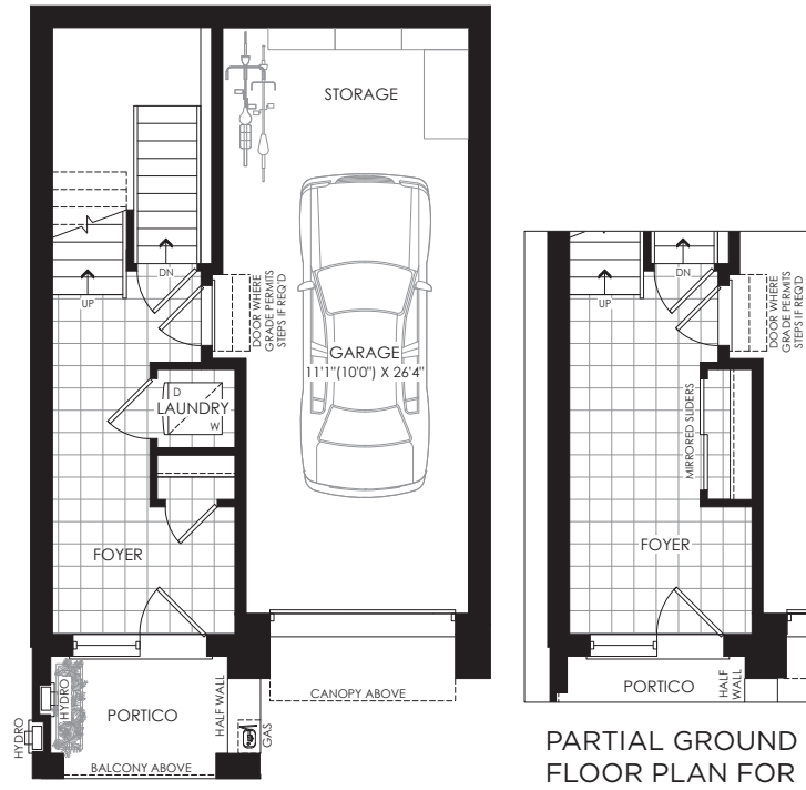
GROUND FLOOR PLAN ELEV. 'A','B'
