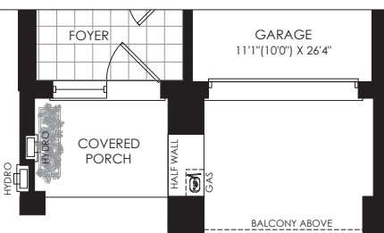
PARTIAL GROUND FLOOR PLAN ELEV. 'G'
