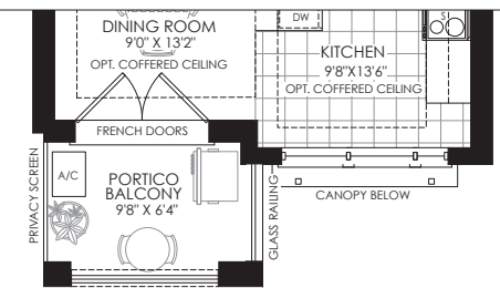
PARTIAL SECOND FLOOR PLAN ELEV. 'C'
