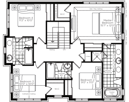
Flex 4 Bed. Second Floor Elev. A
