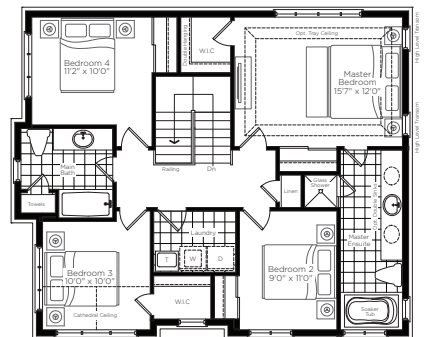
Flex 4 Bed./Laundry Second Floor Elev. A
