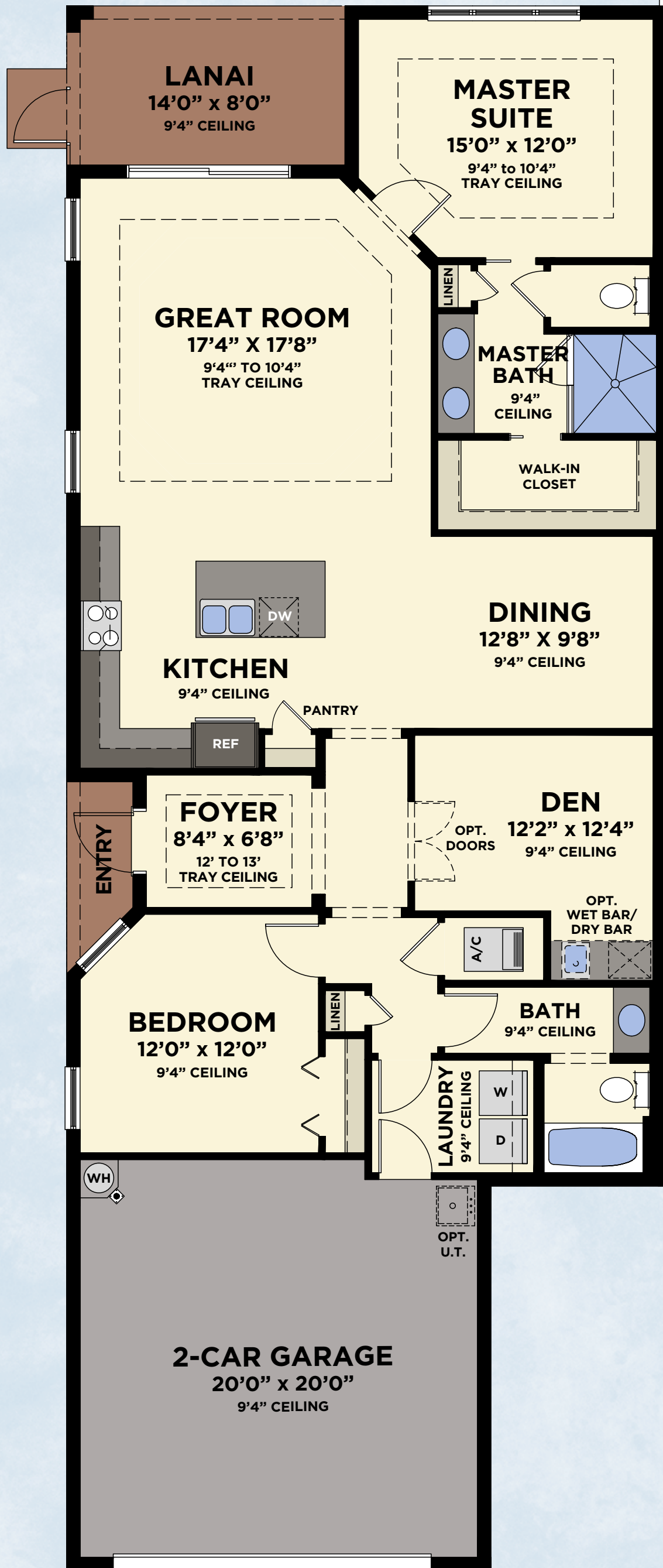
FLOOR PLAN
