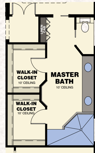
AVAILABLE MASTER BATH VARIATION
