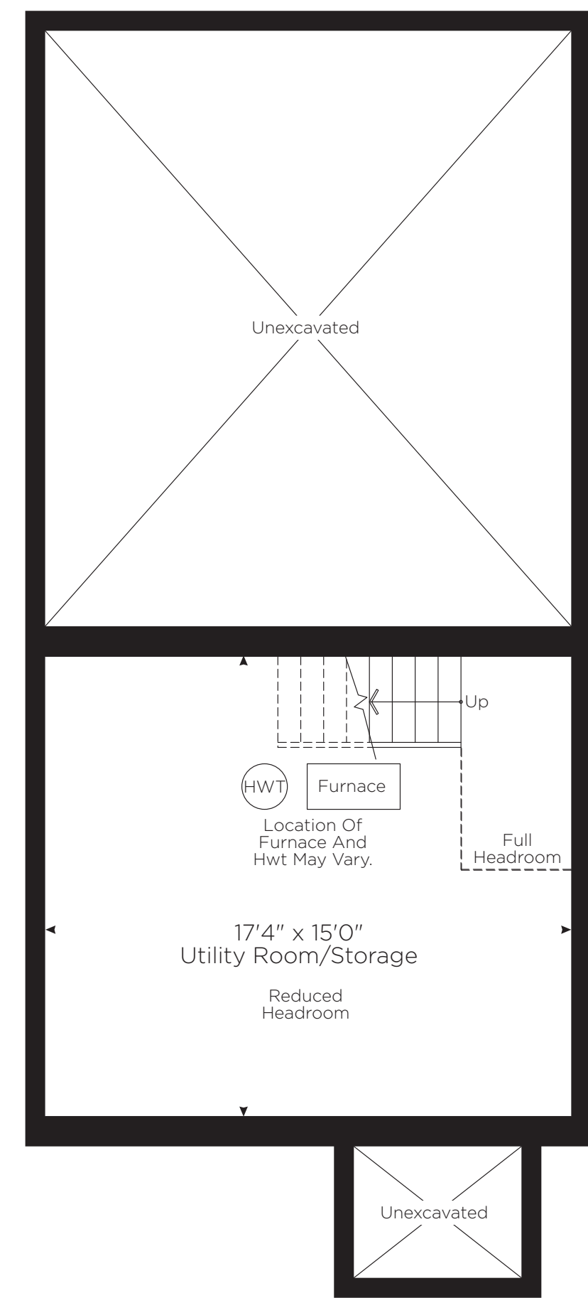
Lower Level
