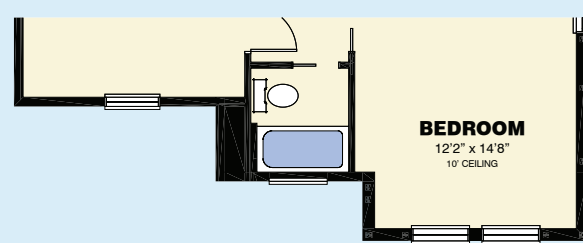
ELEVATION "B" SECOND FLOOR PLAN VARIATION
