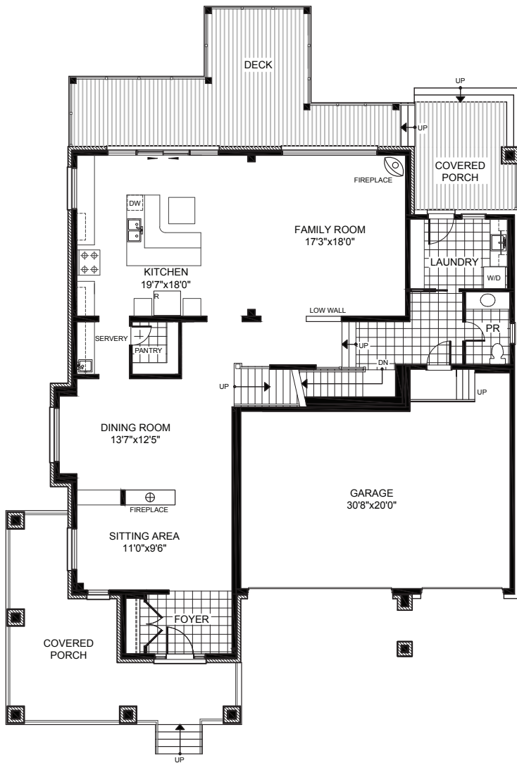
GROUND FLOOR
