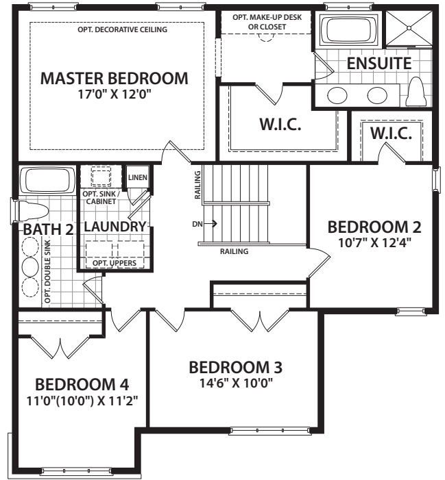
SECOND FLOOR PLAN ELEV. A
