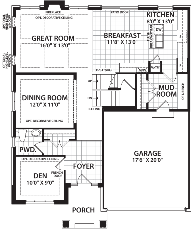
MAIN FLOOR PLAN ELEV. A
