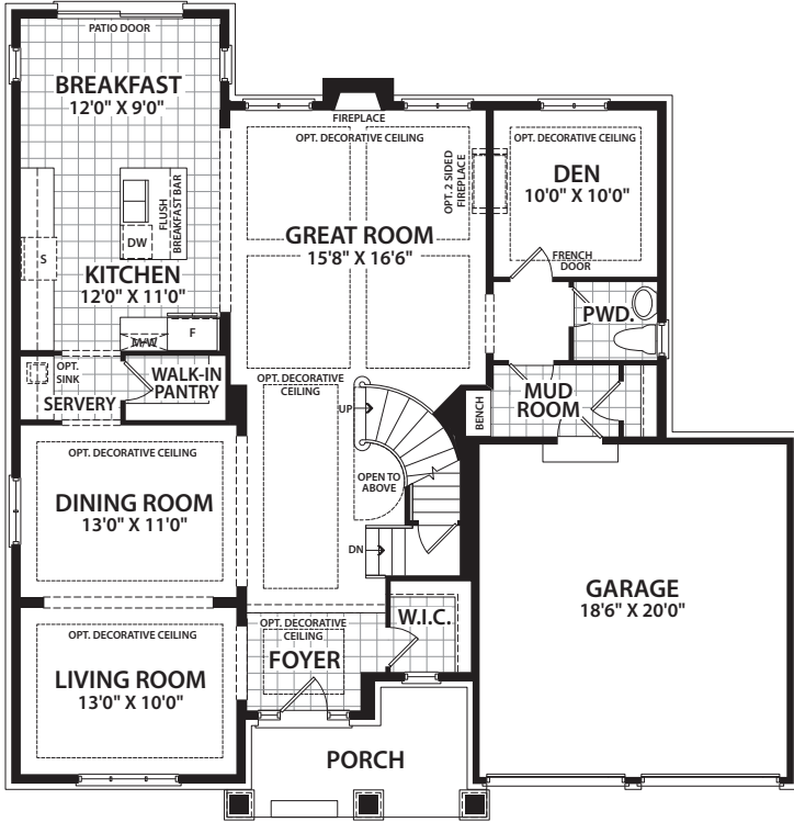
MAIN FLOOR PLAN ELEVATION A
