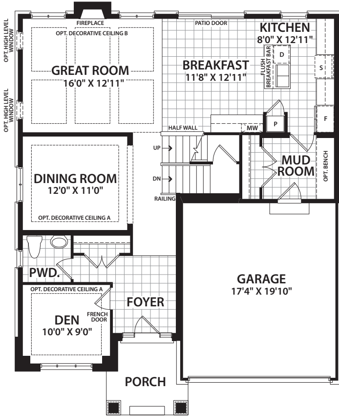
MAIN FLOOR PLAN A
