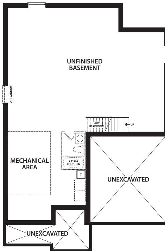
BASEMENT PLAN A & B
