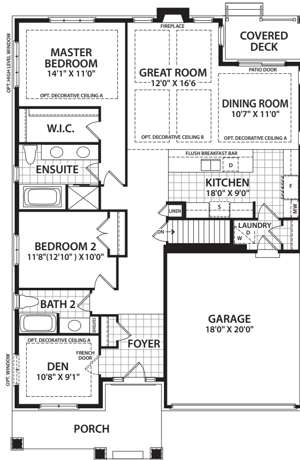
MAIN FLOOR PLAN A
